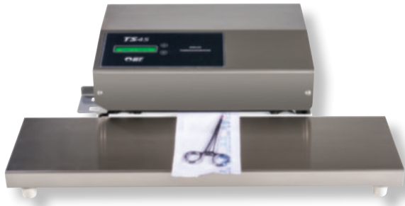
TS 45D sealer with stainless steel support tray
